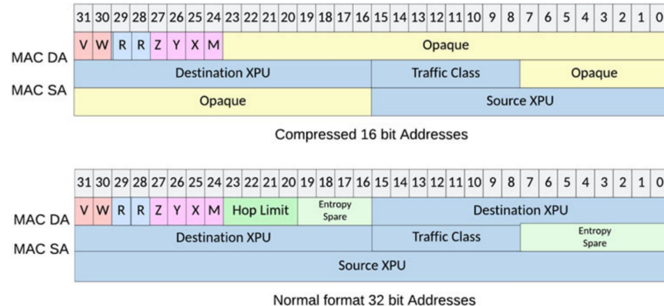
Figure 15: AFH Gen 2 Normal and Compressed Formats
